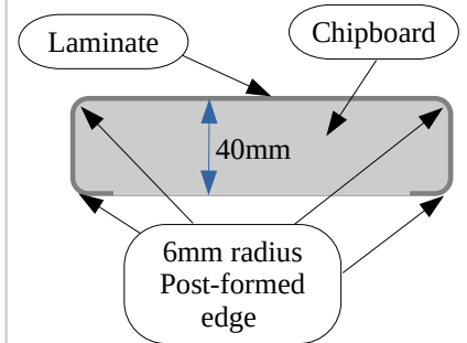
Breakfast Bar Cross Section
