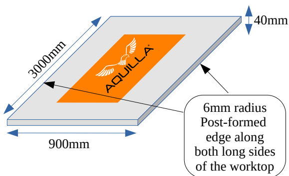
Breakfast Bar (900mm)
