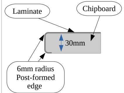
Worktop Cross Section
