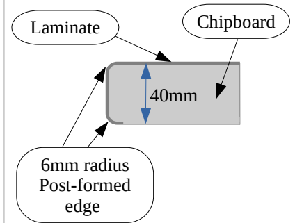
Breakfast Bar Cross Section
