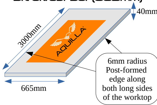
Breakfast Bar (665mm)
